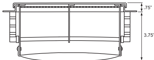
Tube Handle
