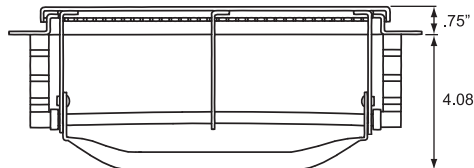
Tube Handle
