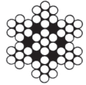
7X7 Construction
