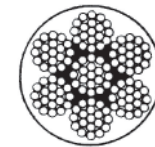
7X19 Construction
